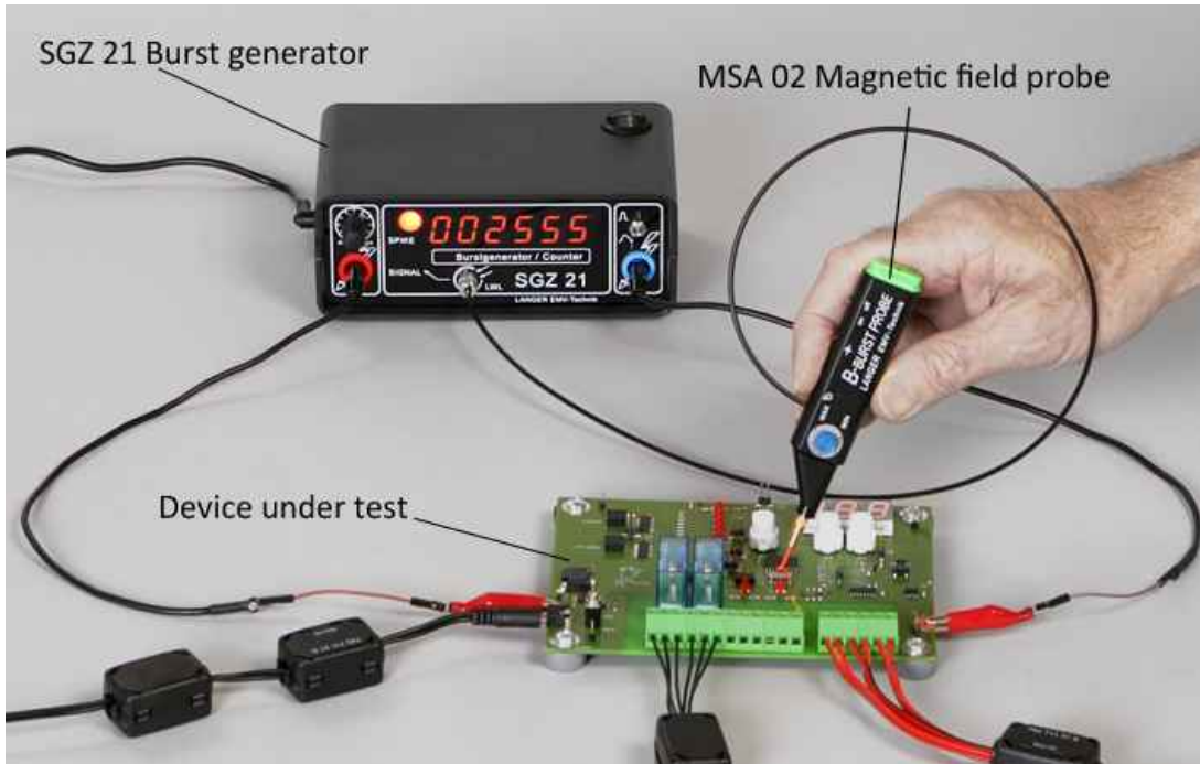
Application with Probe MSA 02-05U
