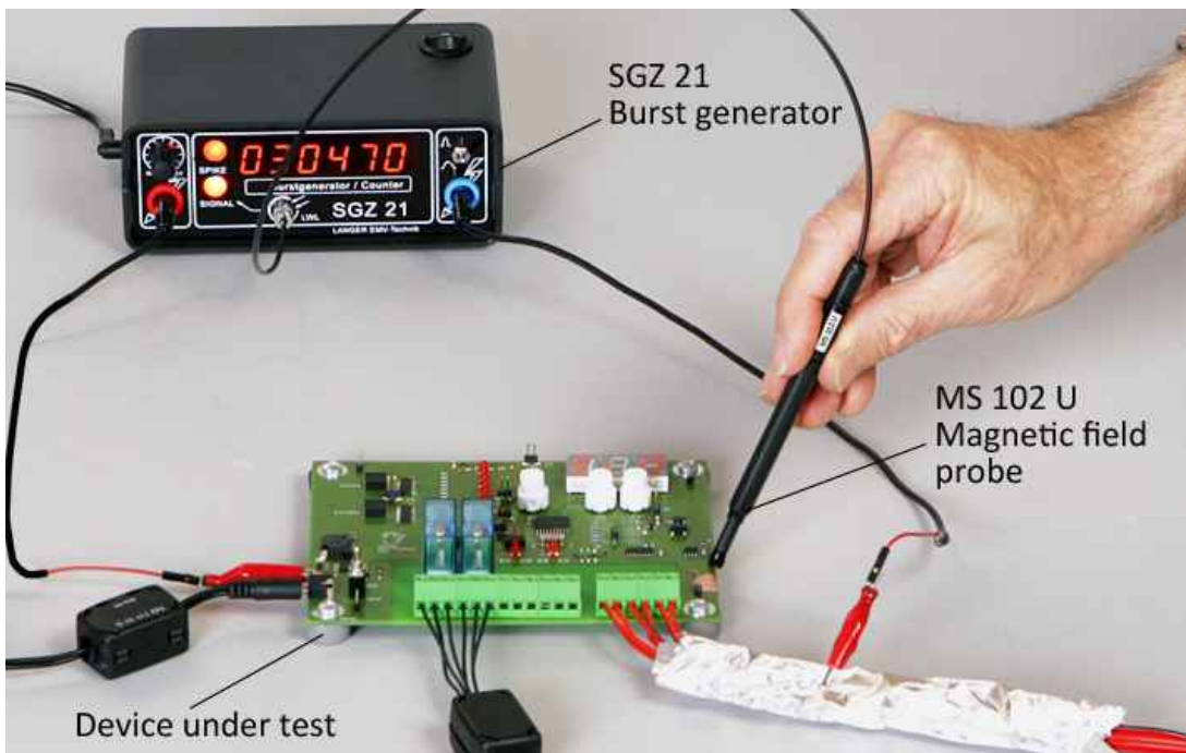
Application with probe MS 102U
