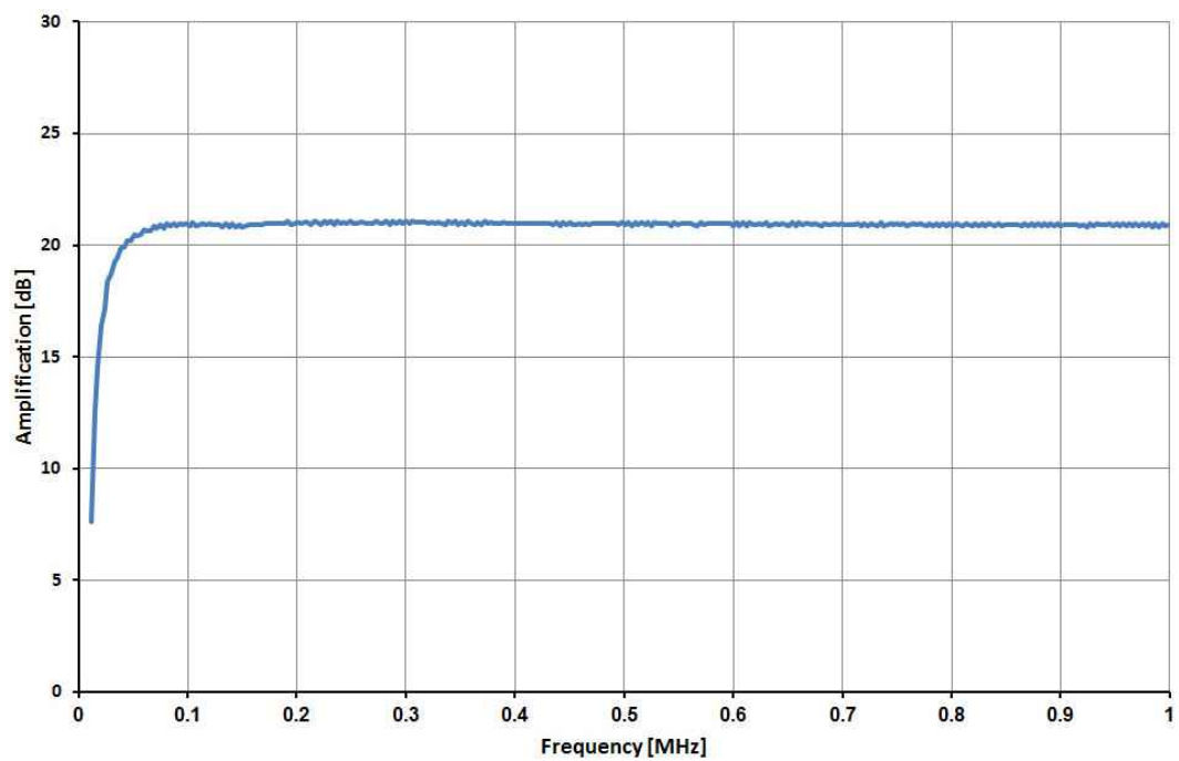
Frequenzgang (Detail)
