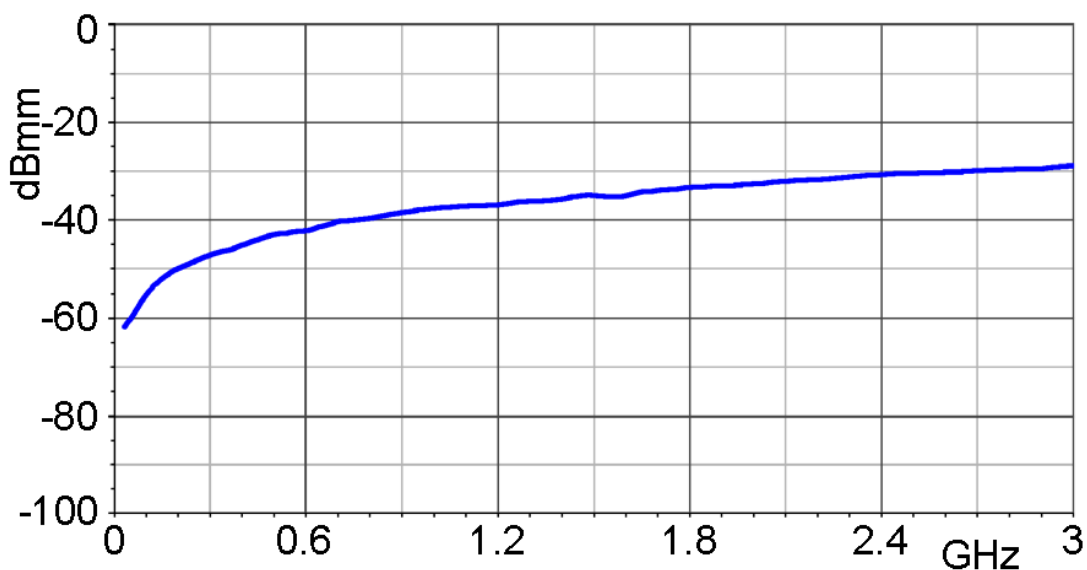
Frequenzgang
