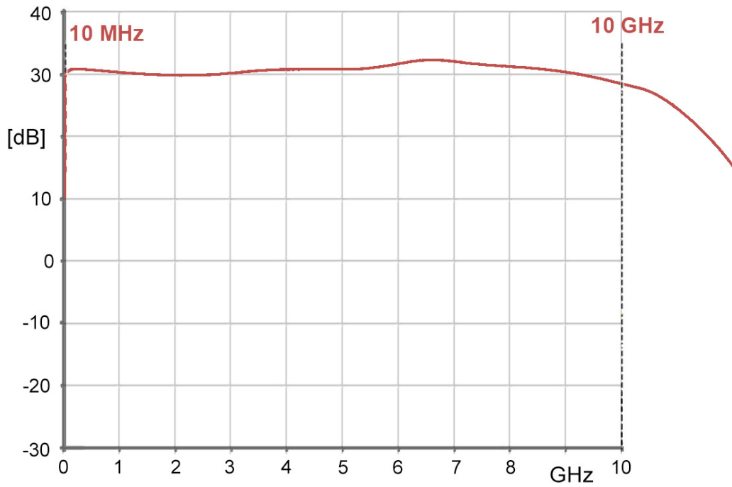
Frequency response
