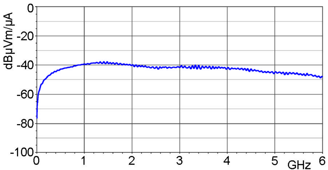
Frequency response [dB \mu\text{V} ] / [dB \mu\text{A}/\text{m} ]
